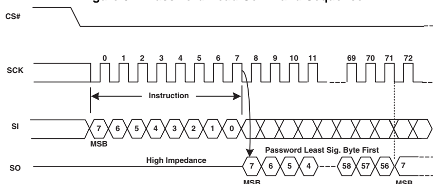
Figure 84. Password Read Command Sequence
