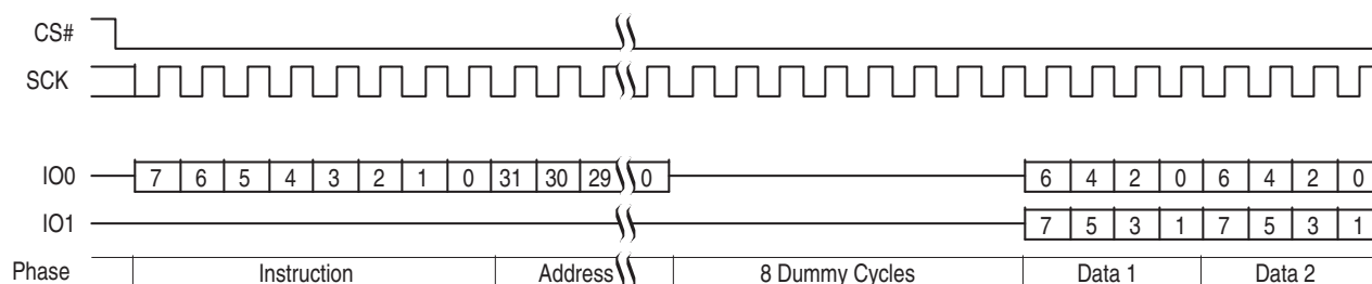
Figure 61. Dual Output Read Command Sequence (4-byte Address, 3Ch or 3Bh [ExtAdd=1, LC=11b])
